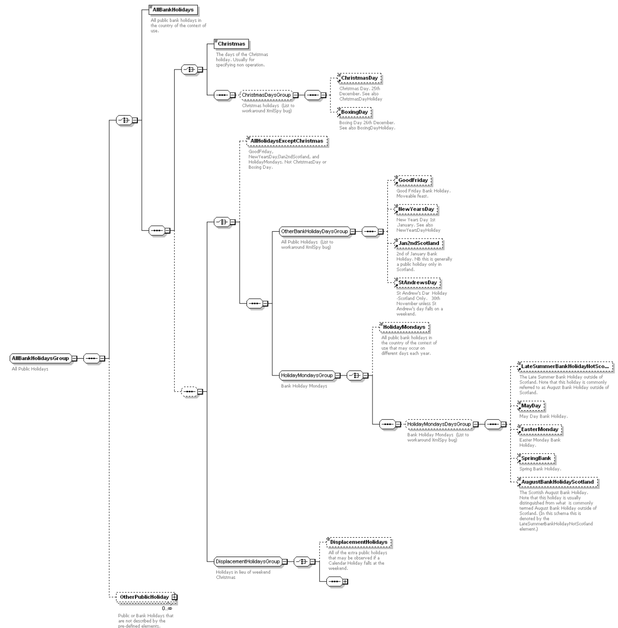
Figure 7-10 – HolidayTypes Element
