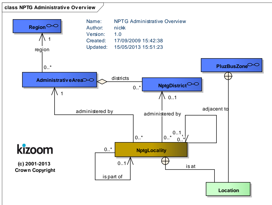
Figure 3-3 – UML Diagram of NPTG Administrative Model: Overview
