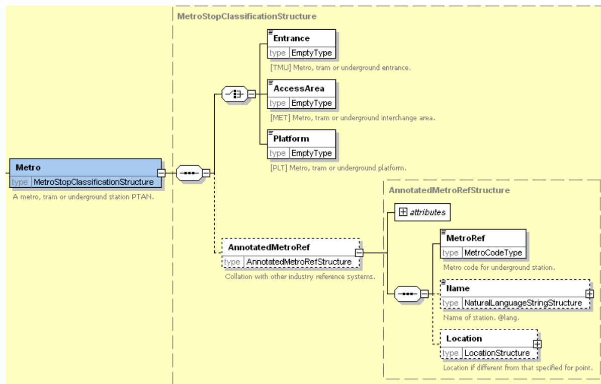
Figure 6-21 – OffStreet / Metro Element
