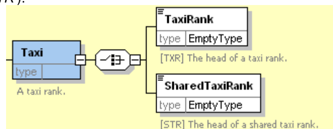
Figure 6-16 – OnStreet / Taxi Element
