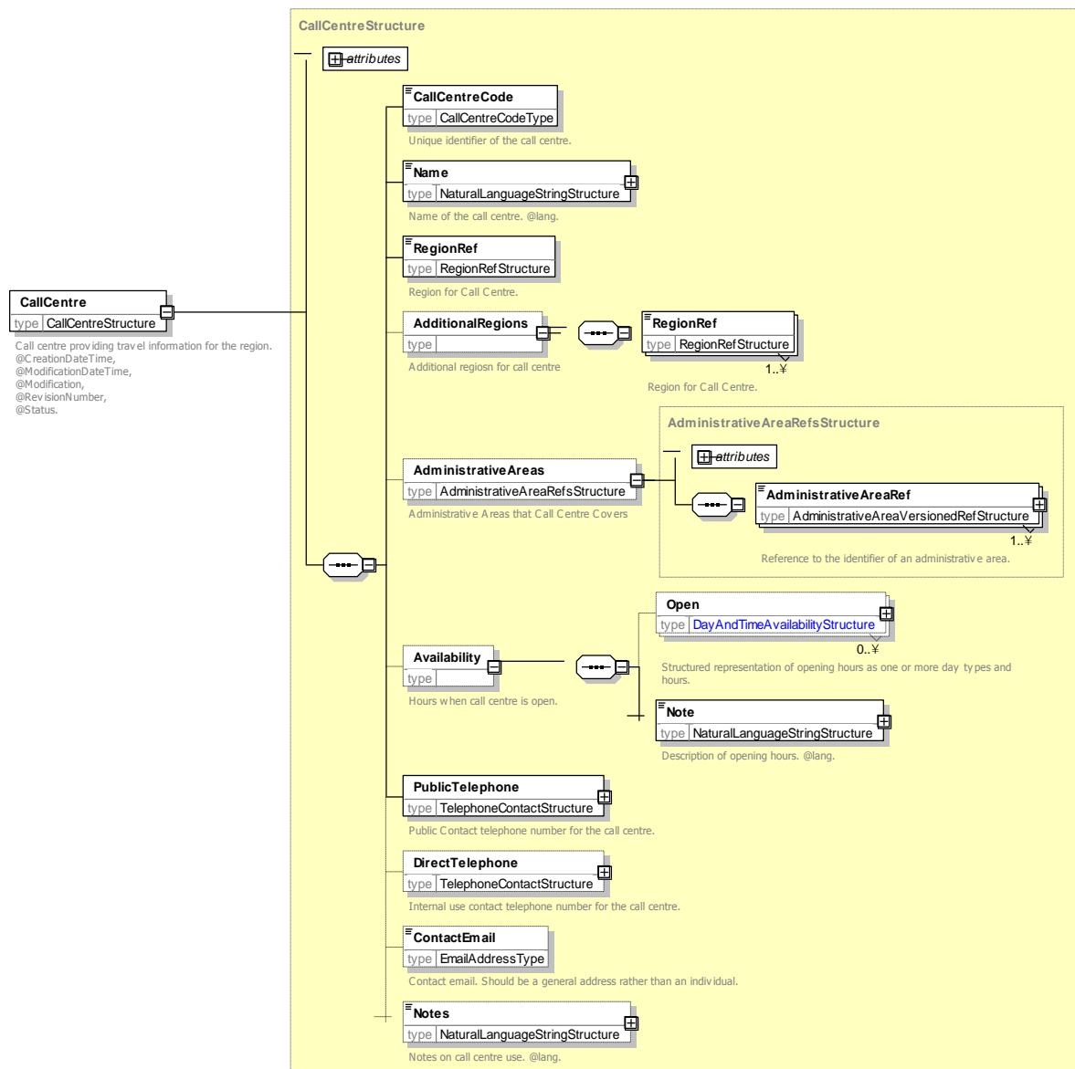
Figure 7-7 – CallCentre Element
