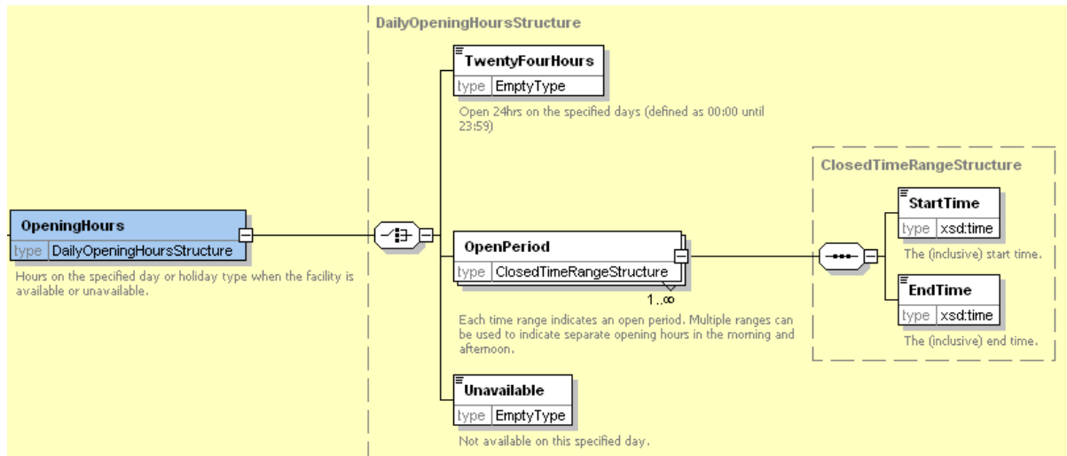
Figure 7-11 – OpeningHours Element
