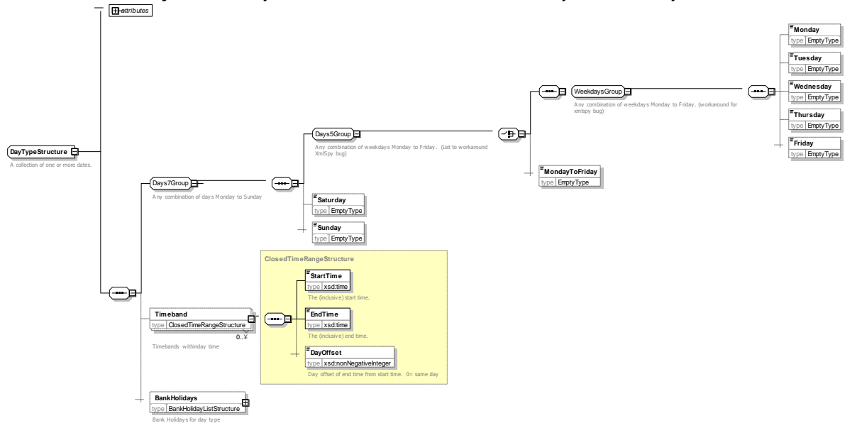
Figure 6-29 – DayType Element
