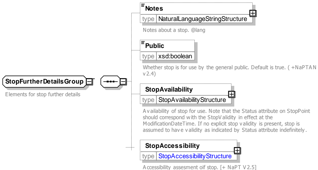
Figure 6-9 – StopFurtherDetailsGroup Group
