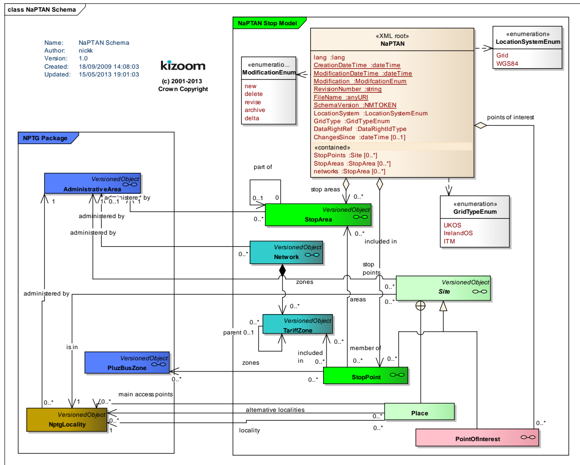
Figure 6-1 – UML Diagram of NaPTAN Schema
